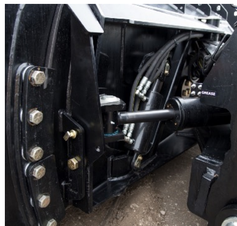
Relocated Tilt Cylinder Reduces Silage Build-up
