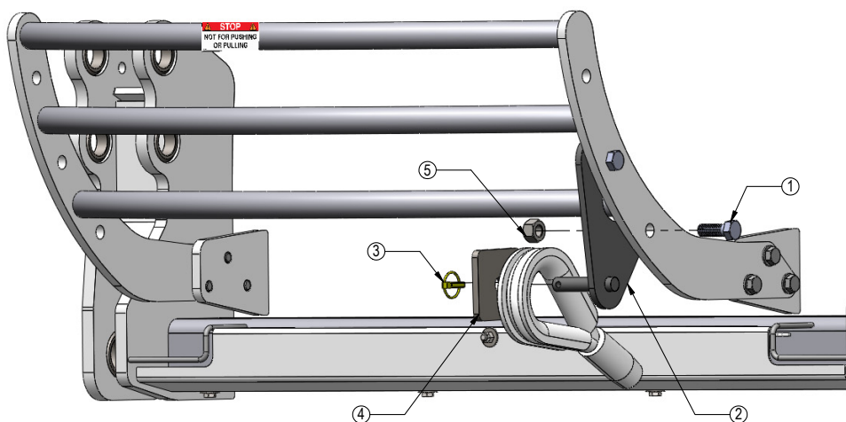
Ag Pro Plus - Tow Cable Support Bracket Assy - 18-19095-A
