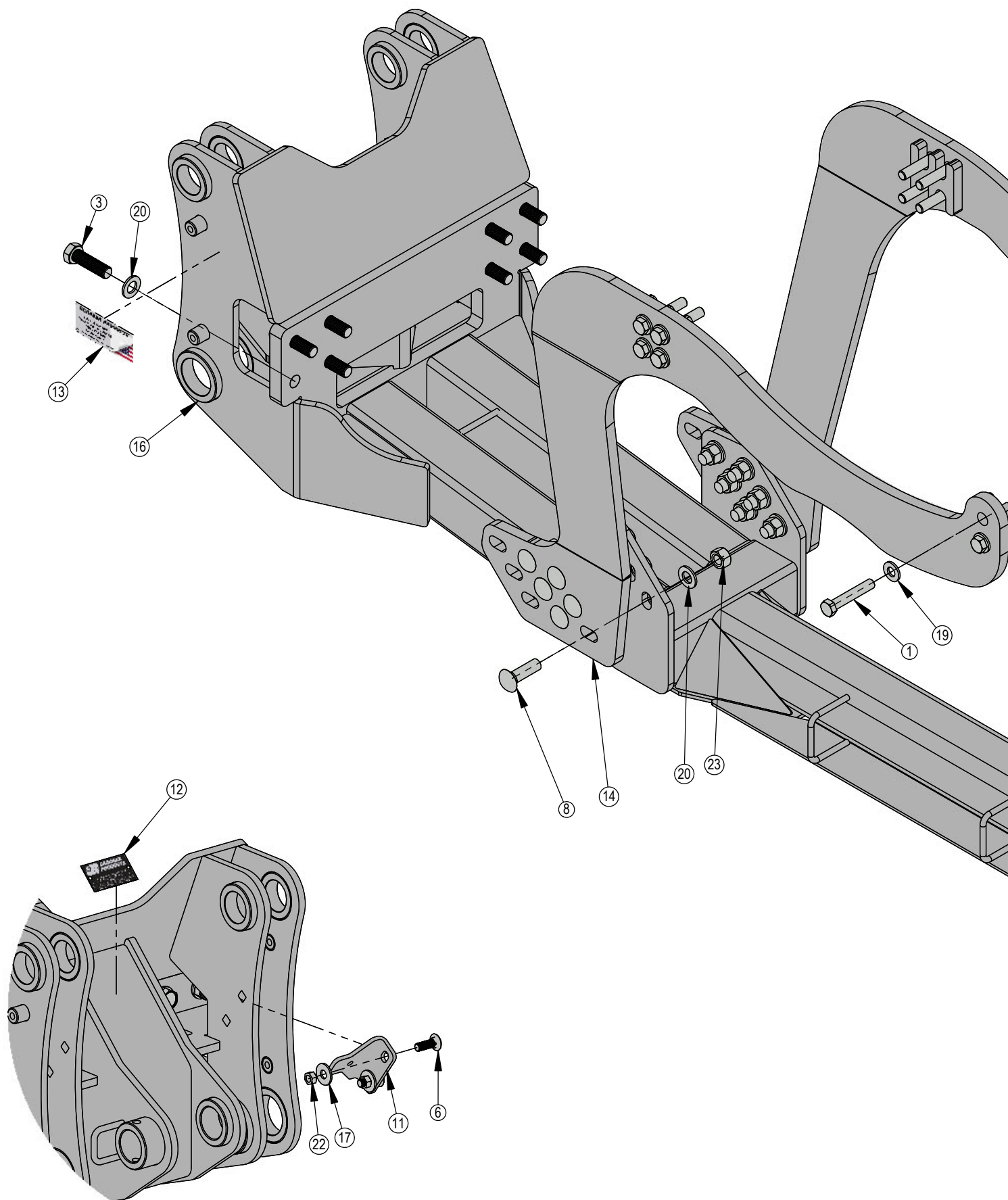
DETAIL A
