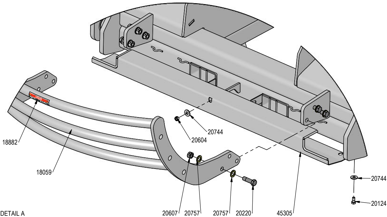
DETAIL A
